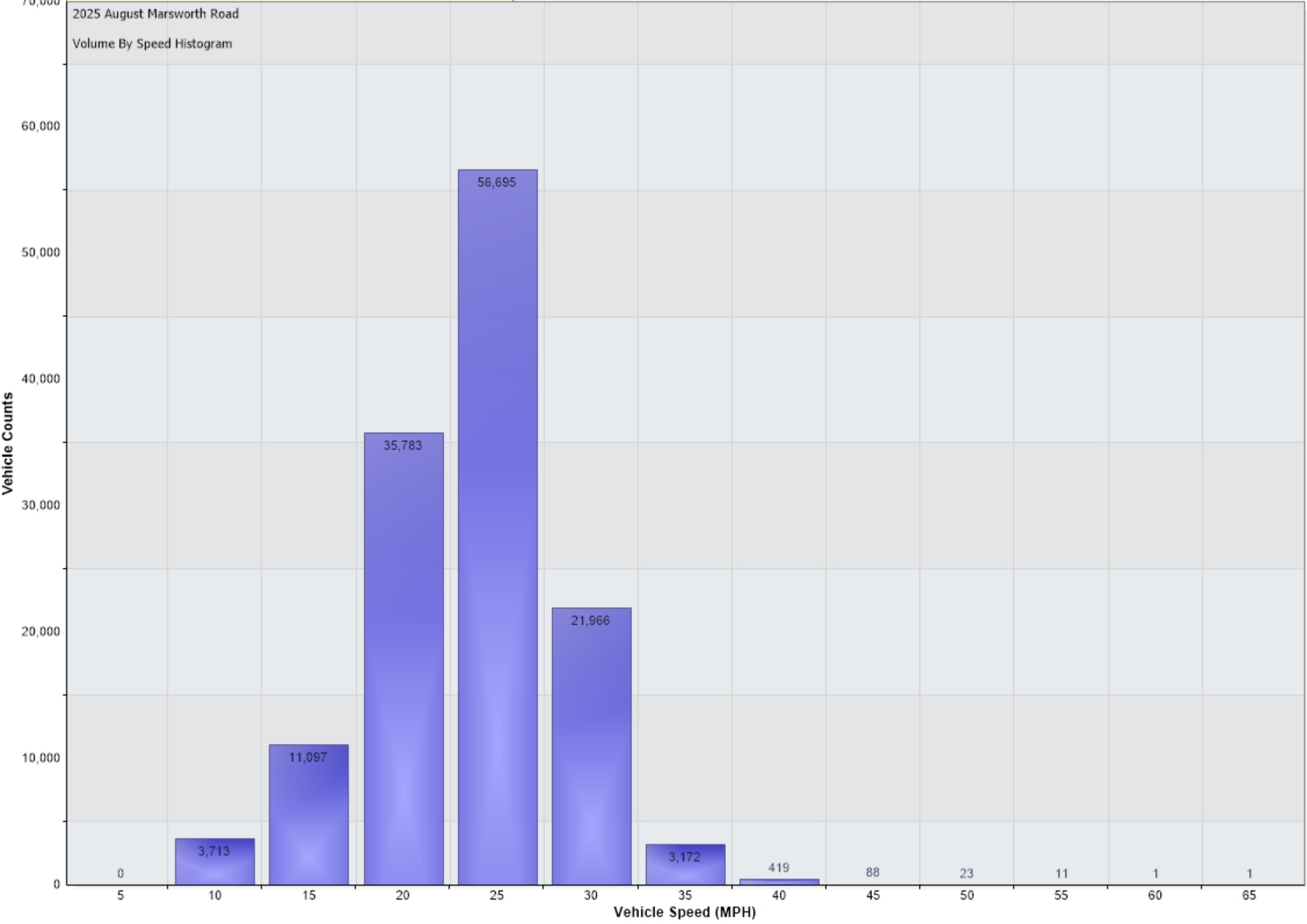
Vehicle Counts Vs. Speed [2025 August Marsworth Road: Incoming]
