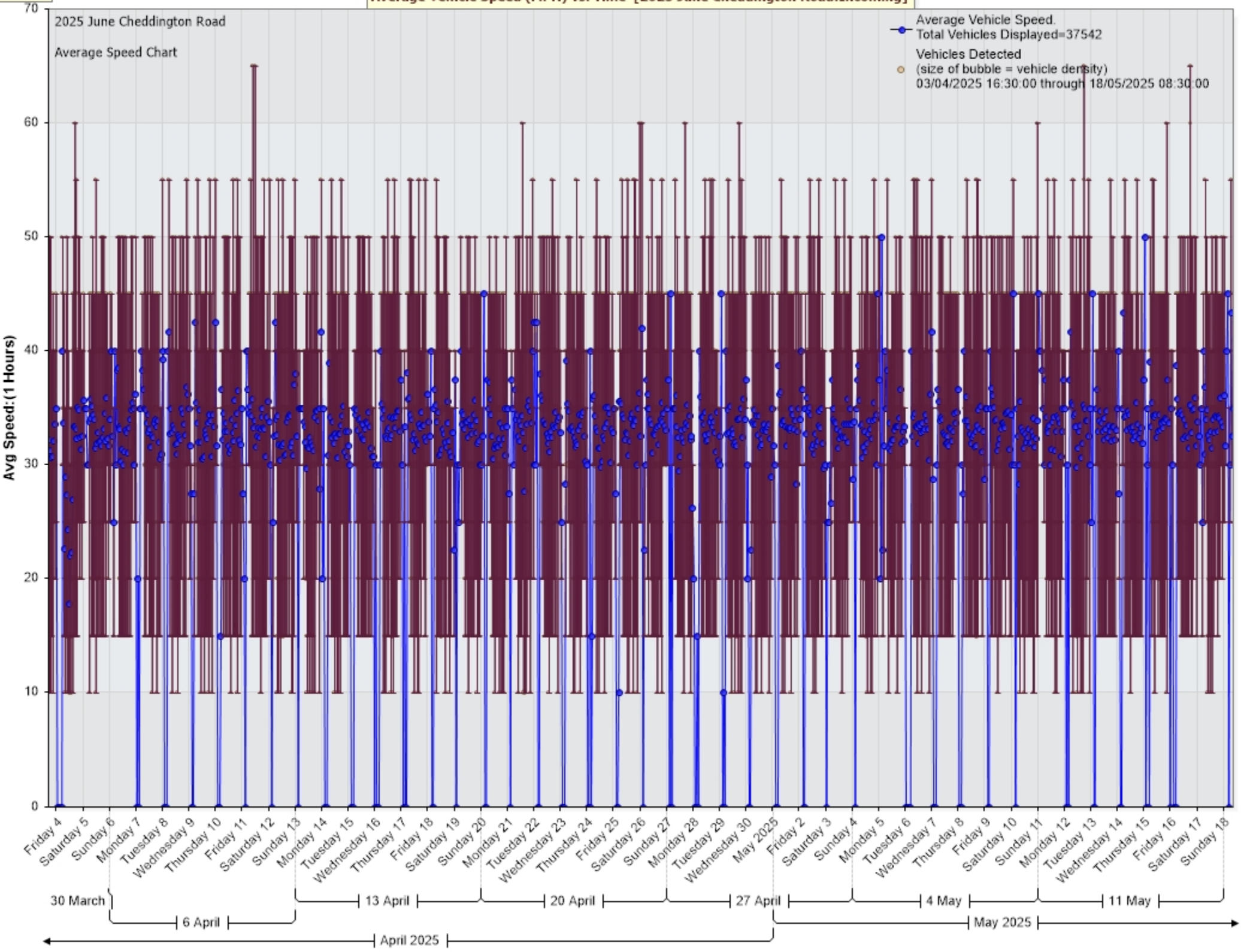
Average Vehicle Speed (MPH) vs. Time [2025 June Cheddington Road:Incoming]
