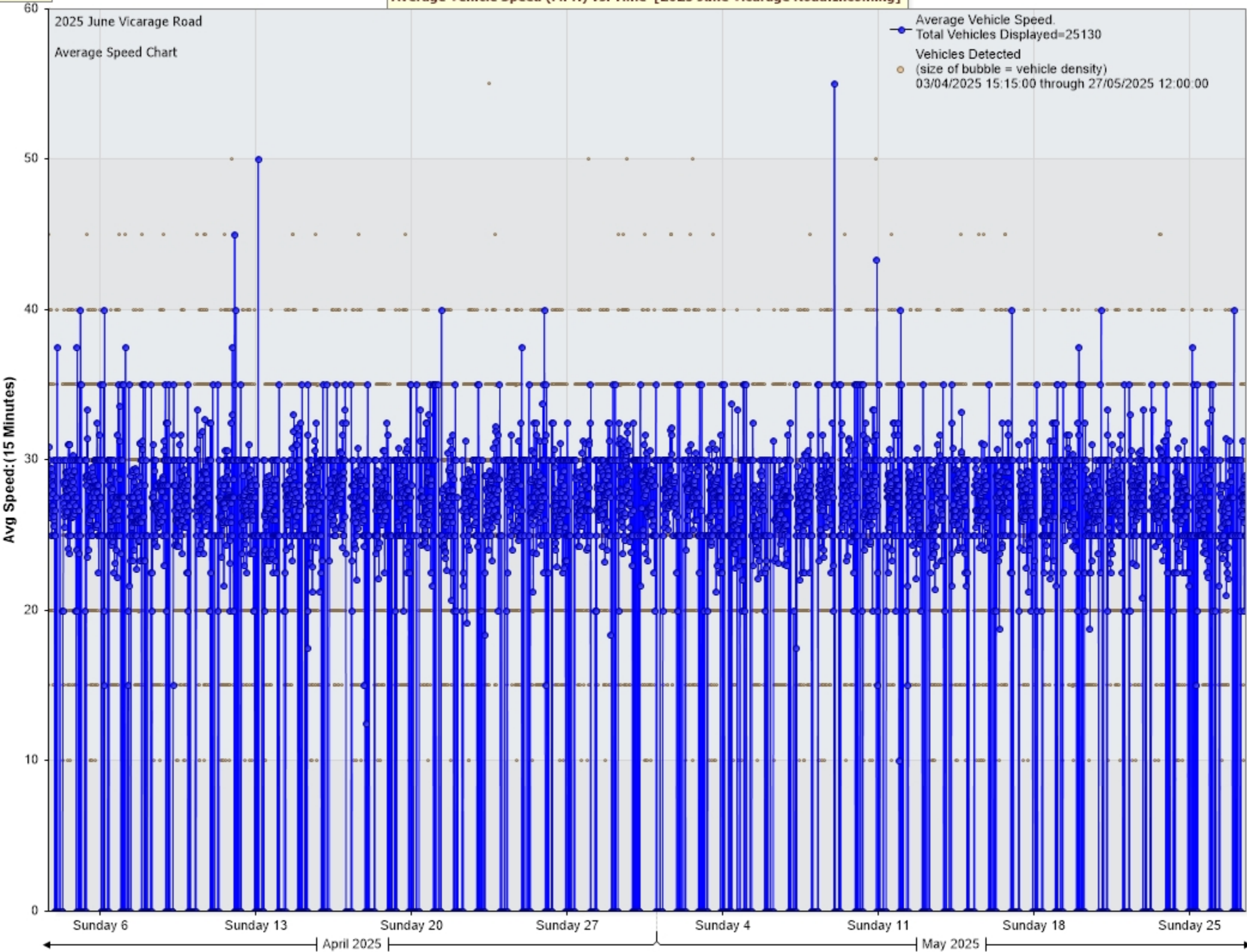
Average Vehicle Speed (MPH) vs. Time [2025 June Vicarage Road:Incoming]
