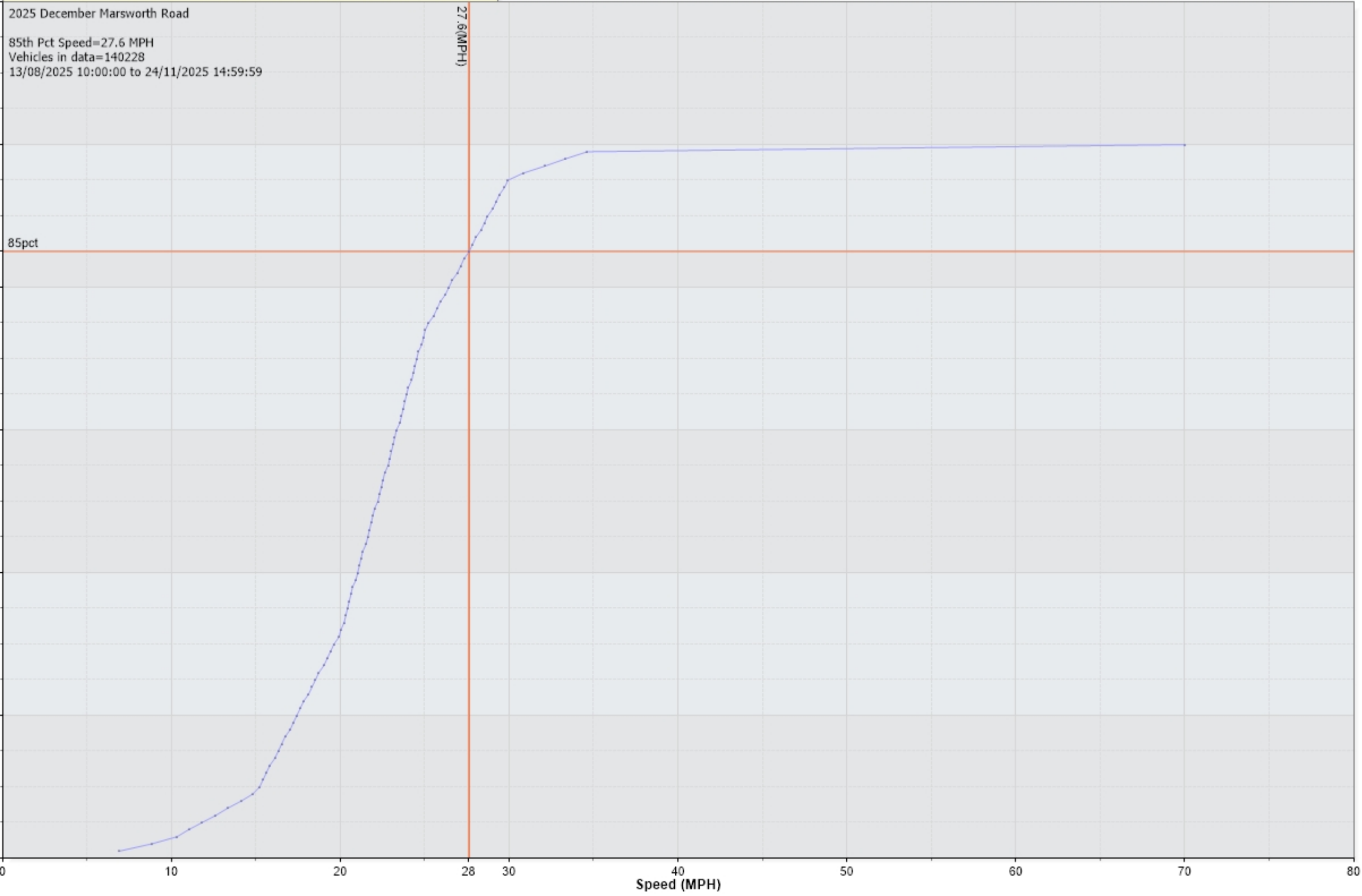
Percentile Counts Vs. Speed for [2025 December Marsworth Road: Incoming]
