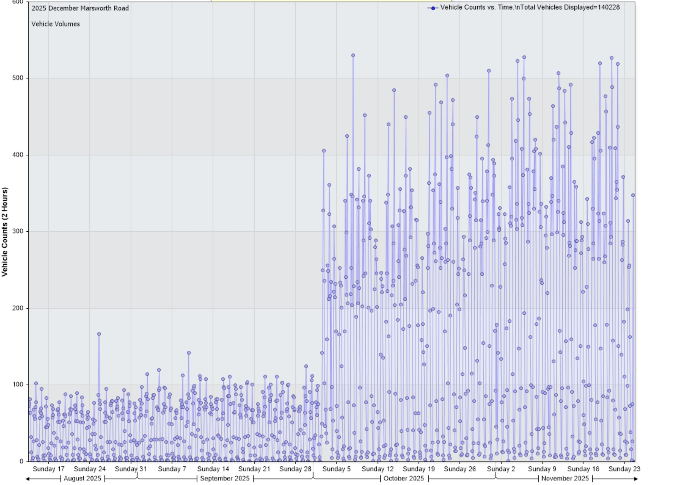
Vehicle Counts vs. Time [2025 December Marsworth Road: Incoming]
