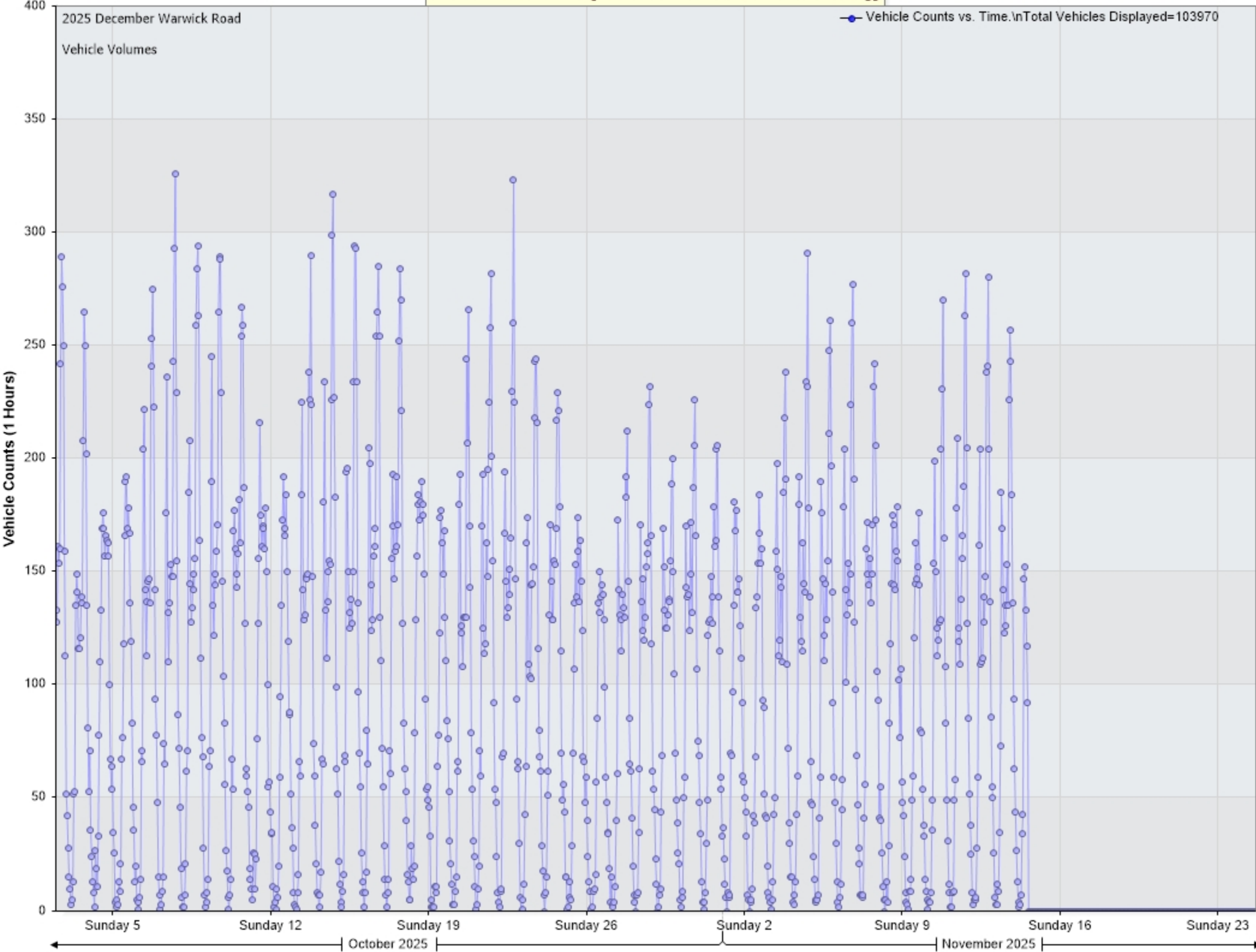
Vehicle Counts vs. Time [2025 December Warwick Road: Incoming]
